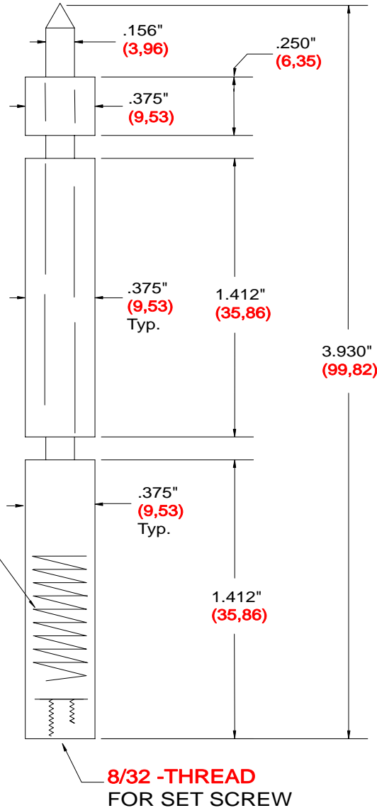
TX-3930-156 TBAA TOP & BOTTOM ALIGNMENT ASSEMBLY
