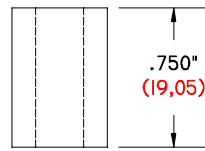
TX-750-500/257 DS .750" (19,05) Long .500" (12,70) O.D. .257" (6,53) I.D.
