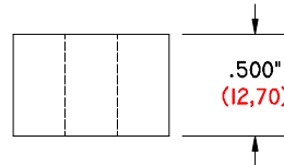
TX-500-750/257 DS .500" (12,70) Long .750" (19,05) O.D. .257" (6,53) I.D.
