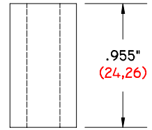
TX-955-500/257 DS .955" (24,26) Long .500" (12,70) O.D. .257" (6,53) I.D.
