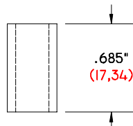
TX-685-375/257 DS .685" (17,34) Long .375" (9,53) O.D. .257" (6,53) I.D.
