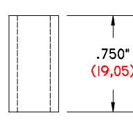
TX-750-375/257 DS .750" (19,05) Long .375" (9,53) O.D. .257" (6,53) I.D.
