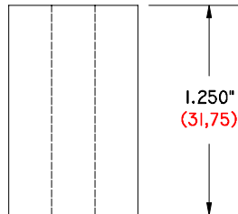
TX-1250-750/257 DS 1.250" (31,75) Long .750" (19,05) O.D. .257" (6,53) I.D.
