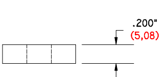
TX-200-750/257 DS .200" (5,08) Long .750" (19,05) O.D. .257" (6,53) I.D.
