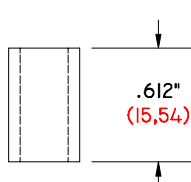
TX-612-375/257 DS .612" (15,54) Long .375" (9,53) O.D. .257" (6,53) I.D.
