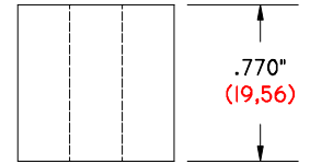
TX-770-750/257 DS .770" (19,56) Long .750" (19,05) O.D. .257" (6,53) I.D.
