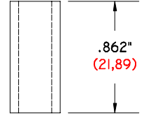
TX-862-375/257 DS .862" (21,89) Long .375" (9,53) O.D. .257" (6,53) I.D.
