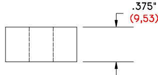
TX-375-750/257 DS .375" (9,53) Long .750" (19,05) O.D. .257" (6,53) I.D.
