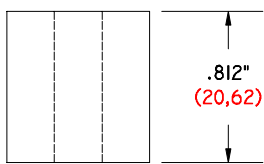
TX-812-750/257 DS .812" (20,62) Long .750" (19,05) O.D. .257" (6,53) I.D.
