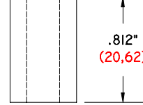
TX-812-500/257 DS .812" (20,62) Long .500" (12,70) O.D. .257" (6,53) I.D.
