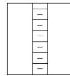
TX-750-750/6-32 DS .750" (19,05) LONG .750" (19,05) Ø O. D. 6-32 THREAD DELRIN SPACER
