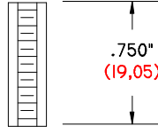
TX-750-250/6-32 DS .750" (19,05) LONG .250" (6,35) Ø O. D. 6-32 THREAD DELRIN SPACER
