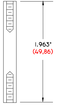
TX-1963-250/8-32 DP 1.963" (49,86) LONG .250" (6,35) Ø O. D. 8-32 THREAD DELRIN POST
