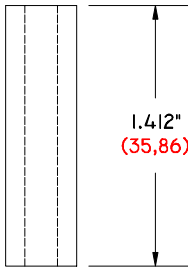
TX-1412-375/170 DS 1.412" (35,86) LONG .375" (9,53) Ø O. D. .170" (4,32) Ø I. D. DELRIN SPACER
