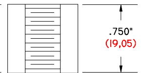
TX-750-750/10-24 DS .750" (19,05) LONG .750" (19,05) Ø O. D. 10-24 THREAD DELRIN SPACER
