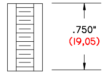
TX-750-375/8-32 DS .750" (19,05) LONG .375" (9,53) Ø O. D. 8-32 THREAD DELRIN SPACER
