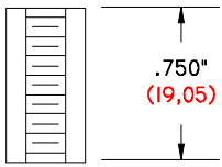
TX-750-312-8-32-DS .750" (19,05) LONG .312" (7,92) Ø O. D. 8-32 THREAD DELRIN SPACER
