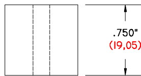
TX-750-750/170 DS .750" (19,05) LONG .750" (19,05) Ø O. D. .170" (4,32) Ø I. D. DELRIN SPACER
