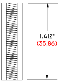
TX-1412-375/8-32 DS 1.412" (35,86) LONG .375" (9,53) Ø O. D. 8-32 THREAD DELRIN SPACER
