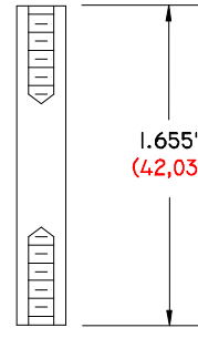
TX-1655-250/8-32 DP 1.655" (42,03) LONG .250" (6,35) Ø O. D. 8-32 THREAD DELRIN POST
