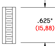
TX-625-250/6-32 DS .625" (15,88) LONG .250" (6,35) Ø O. D. 6-32 THREAD DELRIN SPACER
